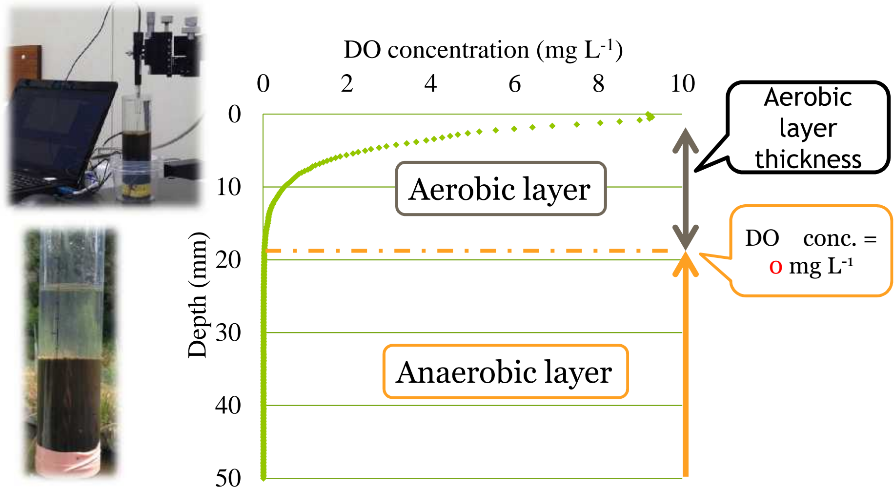
Figure A profile of DO conc. and image for aerobic and anaerobic layer
