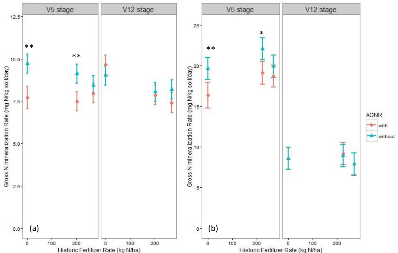
Figure 1. Mean gross N mineralization rate and standard error (vertical bars) in continuous maize for three historic N rates of 0, 202 (long-term AONR) and 269 kg N/ha (highest rate) at the central Iowa site (a) and 0, 224 (rate increment just below the AONR) and 269 (long-term AONR, at the highest rate) at southern Iowa site (b) where either no N or the long-term AONR fertilizer rate was applied; determined at the V5 (5 collared leaves) and V12 (12 collared leaves) maize growth stage. ** indicates the difference between zero and AONR fertilizer application is significant at P = 0.05 and * indicates the differences are significant at P = 0.10 .
